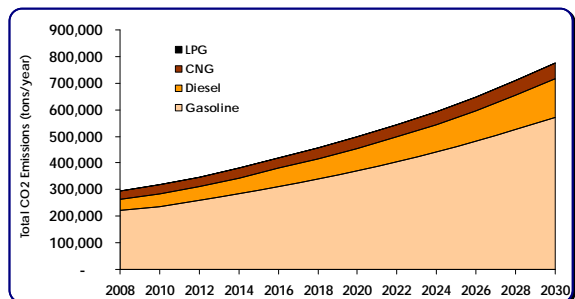
Carbon Dioxide
