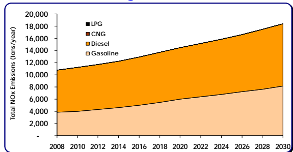
Nitrogen Oxides
