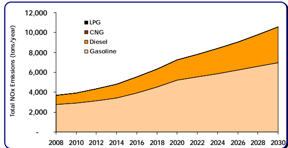
Nitrogen Oxides
