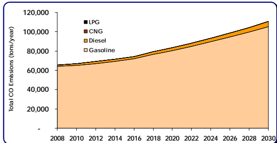
Carbon Monoxide
