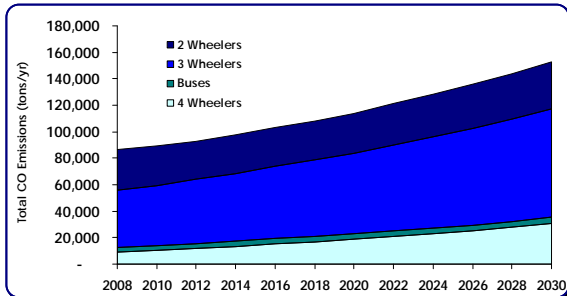
Carbon Monoxide
