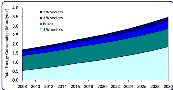
Total energy consumption by category
