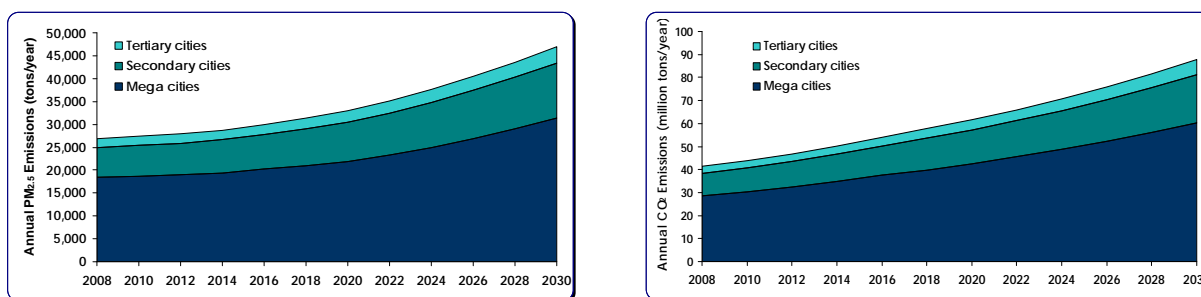
Figure 8: Annual total emissions for PM 2.5 and CO 2 for all the cities combined
