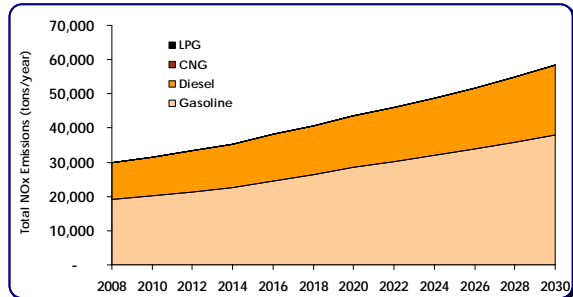
Nitrogen Oxides
