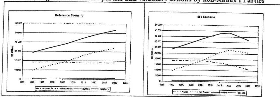
Figure 3. Reference scenario form the 2009WEO and mitigation scenario that includes current pledges from Annex I parties and voluntary actions by non-Annex I Parties
