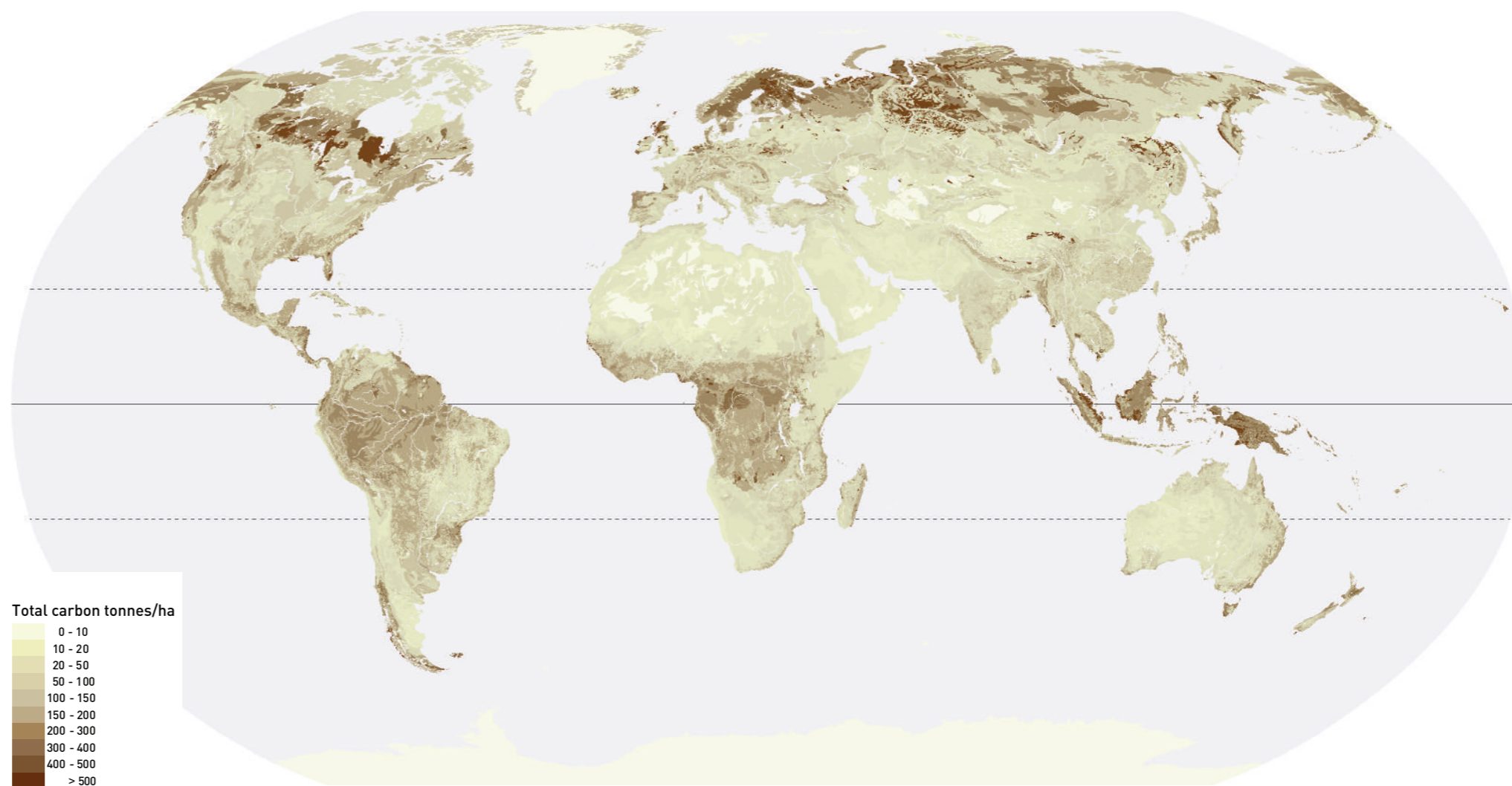
Carbon storage in terrestrial ecosystems.
