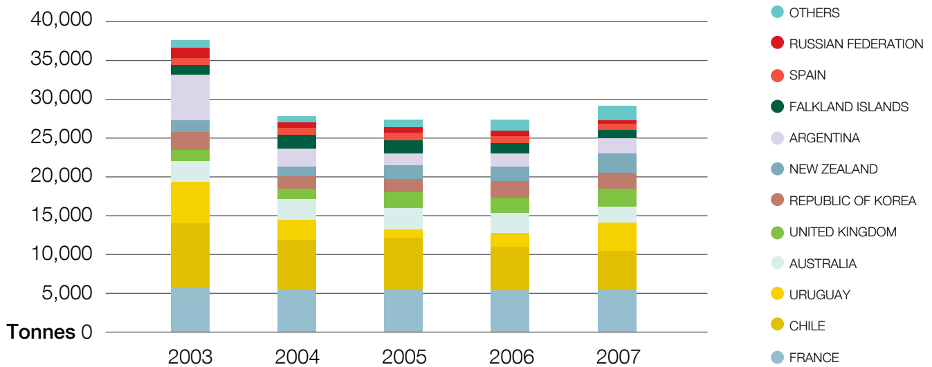
Figure 5 Global catch of toothfish ( Dissostichus species) in tonnes by country. 70
