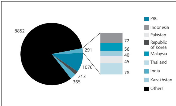
Figure 2.12 (a): Electricity Consumption (TWh), 1999
