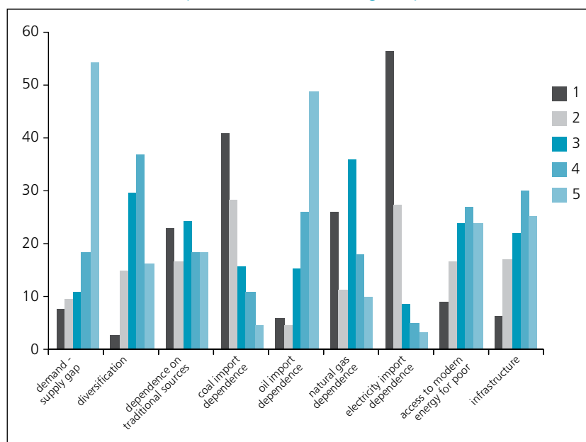
Figure 3.7: Key Energy Security Concerns in Asia and the Pacific Countries (1 is lowest and 5 is highest)
