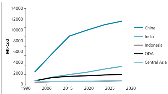
Figure 2.23: CO 2 Emissions Projections (Mt-CO 2 )
