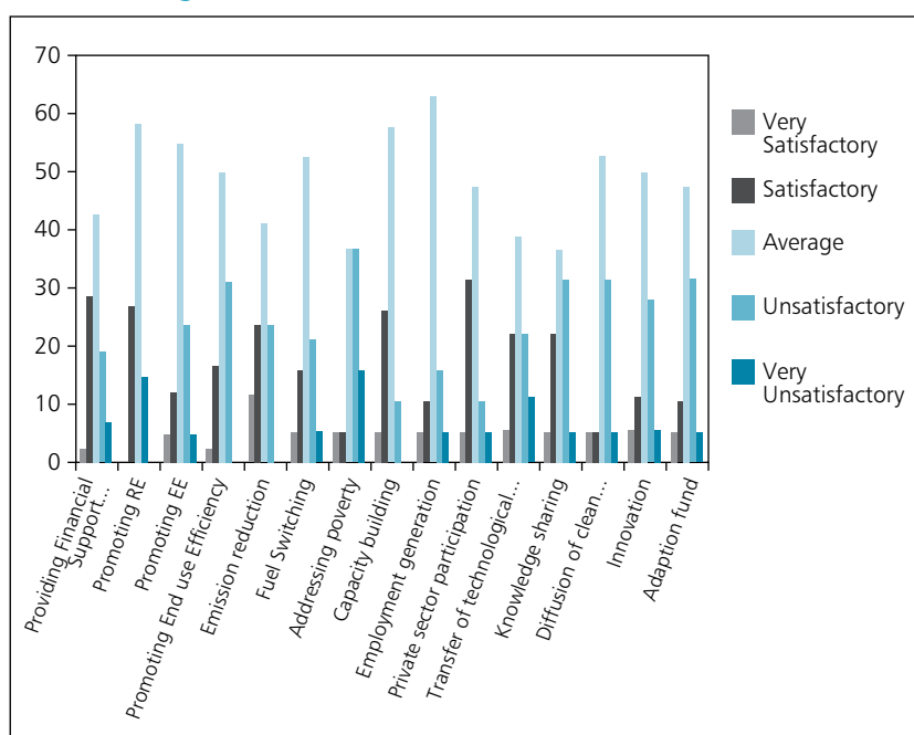
Figure 6.6: Assessment of CDM Performance
