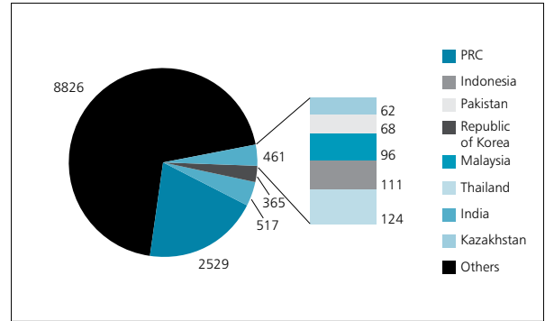
Figure 2.12 (b): Electricity Consumption (TWh), 2006
