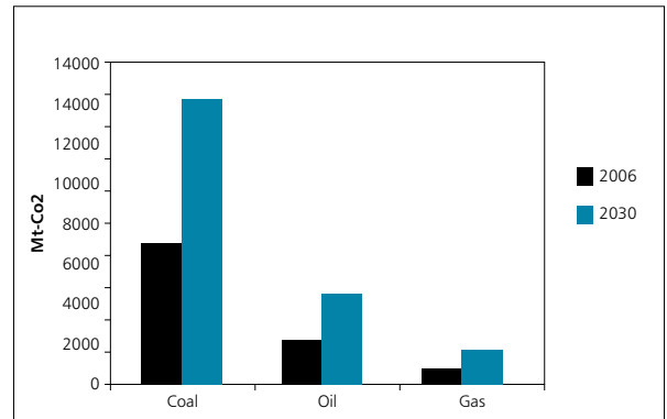
Figure 2.24: Region's CO 2 Emissions by Fuel, 2006 and 2030
