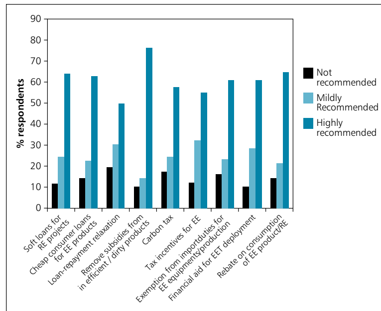
Figure 4.8: Financial Incentives/Disincentives for Energy Efficiency/Renewable Energy Promotion
