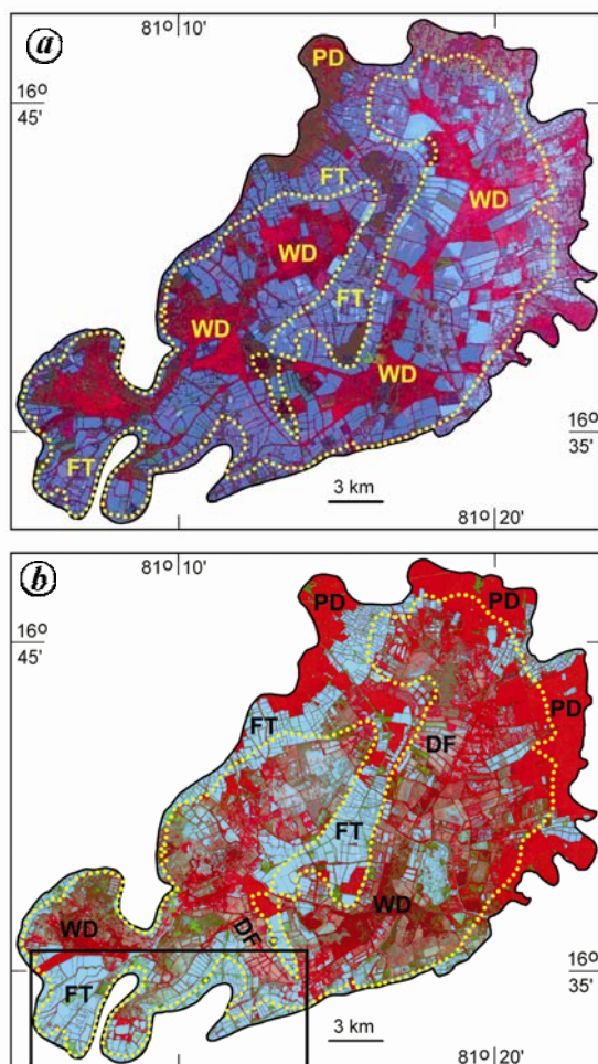
Figure 2. Status of the Kolleru lake area in 2004 (a) and 2008 (b) within the 5 foot ( \approx 1.5 \text{ m} ) contour. Yellow coloured dotted line in both (a) and (b) represents the 3 foot ( \approx 0.9 \text{ m} ) contour. FT: Fish tanks in blue colour with characteristic embankments; PD: Area under paddy cultivation; WD: Weed in mottled brownish-red; DF: Drained fish tanks with their embankments still intact, in red colour due to weed growth. Area enclosed in black rectangle in (b) is enlarged in Figure 3.
