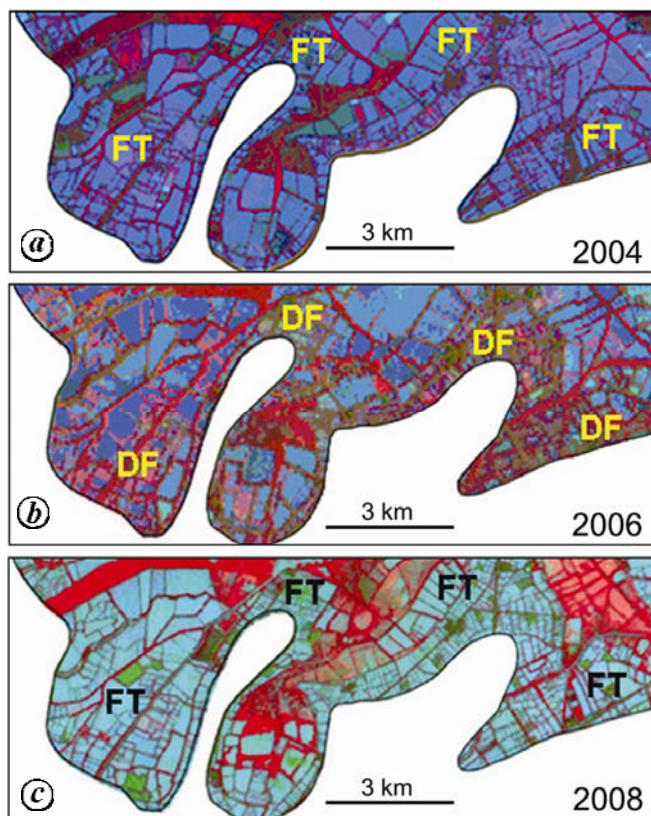
Figure 3. Southeastern part of the Kolleru lake. (See its location in Figure 2 b.) Fish tanks (FT) in the 2004 image (a) were later drained during Operation Kolleru and hence appeared in the 2006 image (b) in red colour (drained fish tank (DF)) due to weed growth. FT reappeared in the area as seen in the 2008 image (c).
