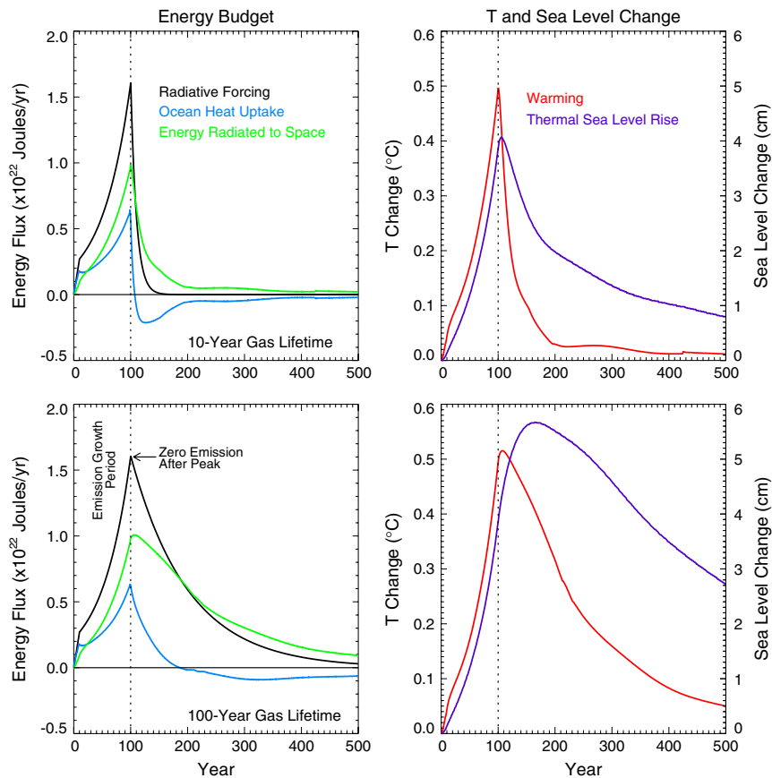
Fig. 3. Energy budget terms calculated by the Bern 2.5CC model for an increase in radiative forcing from 0 to 1 W/m 2 over 100 y and a subsequent decline in that forcing determined by a 10-y adopted gas lifetime ( Upper ) or 100-y gas lifetime ( Lower ). The left panels show instantaneous terms in the energy budget, whereas the right panels present the computed warming and sea level rise due to ocean thermal expansion only. The black lines show radiative forcing, whereas the pale-blue lines show ocean heat uptake. The difference between radiative forcing and ocean heat uptake is also shown as the pale-green lines, and this represents the energy emitted by the Earth–atmosphere system to space in response to the forcing. The modeled atmospheric temperature responses are represented by the red lines in the right panels, which track the instantaneous energy emitted by the Earth–atmosphere system.
