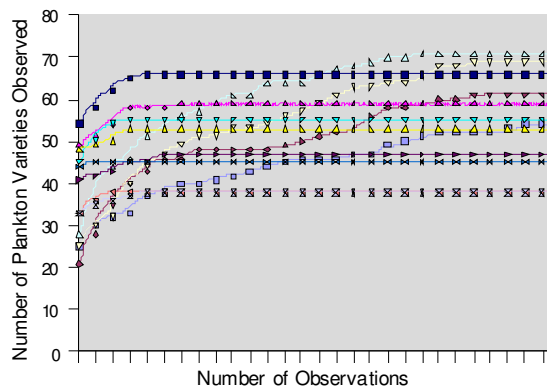
Fig. 1: Figure showing the saturation curve for each water body. Irrespective of the nature of the water body the saturation in plankton diversity is obtained indicating that no further increase in the plankton diversity would be achieved with further increase in the number of observations
