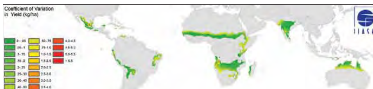
Figure 81. Modeled coefficient of variation in attainable yield for lowland groundnut with a 90-day growing period.
