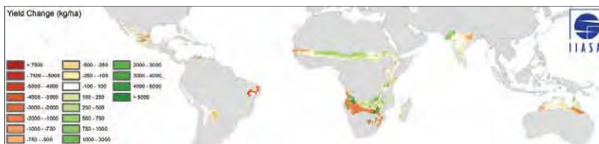
Figure 110. Maize yield changes in the 2020s simulated with AEZ using HadCM3 and SRES A2.
