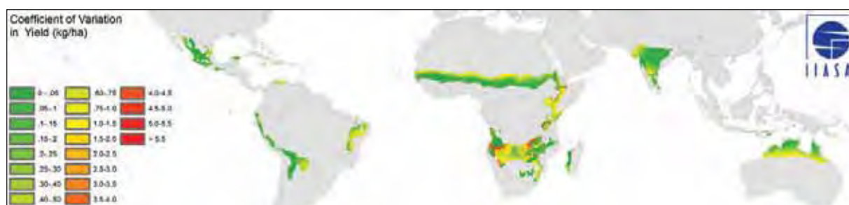
Figure 11. Modeled coefficient of variation in attainable yield for lowland maize with a 90-day growing period.
