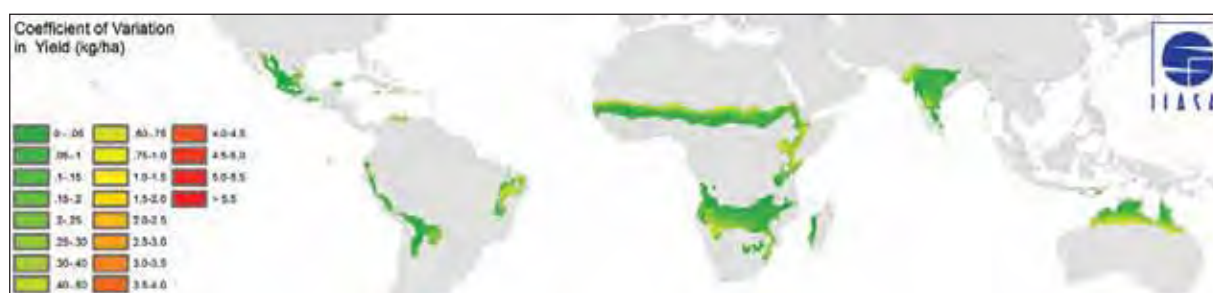
Figure 74. Modeled coefficient of variation in attainable yield for pearl millet with a 90-day growing period.
