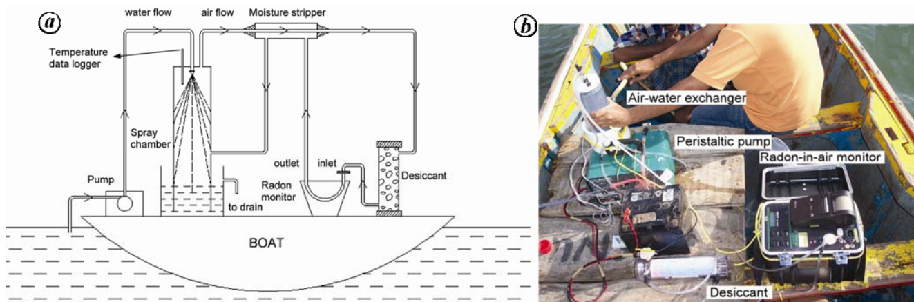
Figure 2. a, Schematic sketch of surface water 222 Rn monitoring system; b, In situ measurement of 222 Rn in coastal water.
