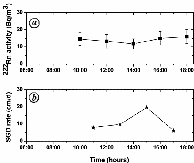
Figure 6. a, Temporal variation of 222 Rn and b, estimated SGD rates in Vizhinjam coastal waters during 27 November 2007 ( 222 Rn activities and SGD rates are expressed as integrated values for a 2 h period).
