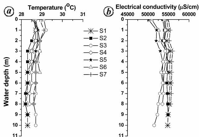
Figure 3. Vertical profiles of water temperature (a) and electrical conductivity (b) in Vizhinjam coastal waters during November 2007.
