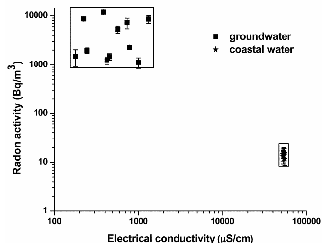
Figure 4. Comparison of ^{222}\text{Rn} activities in groundwater and coastal waters, Vizhinjam, Kerala.
