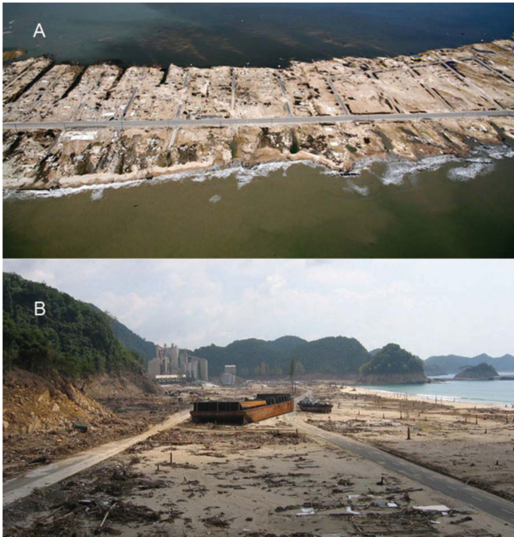
Figure 1 (A) Storm surge destruction as caused by September 2008's Hurricane Ike, Bolivar Peninsula, Texas, USA. (B) Tsunami destruction as caused by the December 2004 Indian Ocean Tsunami, Aceh, Indonesia. Buoyancy is a surprisingly powerful force as evidenced by the barge. In
