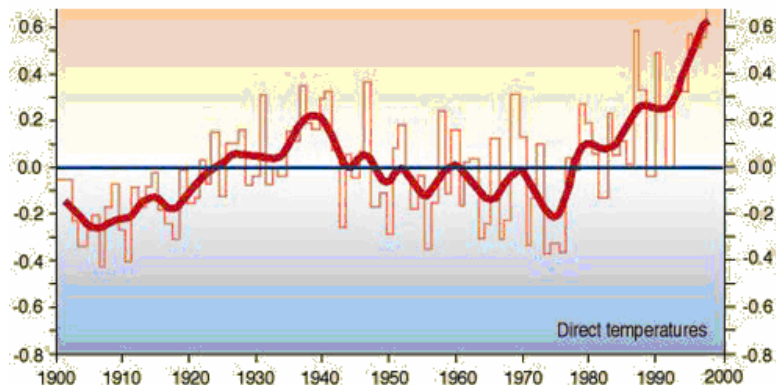
Figure 6: Temperature Curves in Africa during the Twentieth Century
