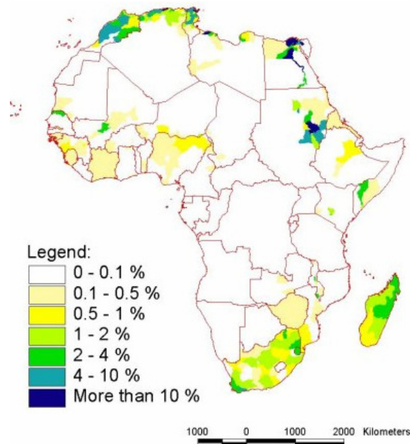
Figure 3: Irrigated Areas in Africa
