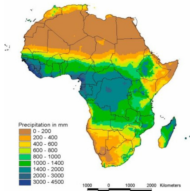
Figure 2: Average Annual Precipitation
