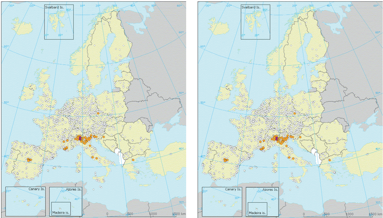
Map 2.3 Selected days during the ozone episode at the end of June 2008: observed and modelled maximum 1-hour ozone concentrations
