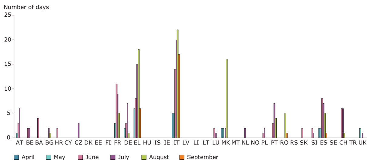
Figure 2.1 Number of days on which at least one exceedance of the one-hour threshold value was observed per country and per month during the summer of 2008 (only countries that submitted data are shown)
