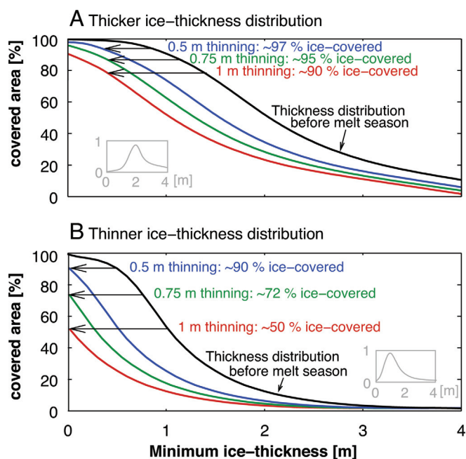
Fig. 2. Comparison of the impact of a certain amount of summer melt on the ice-covered area for two different ice-thickness distributions. The black line shows which percentage of a certain area is covered by ice that is thicker than the ice thickness indicated along the x axis at the beginning of the melt season (cumulative ice-thickness distribution). A shows a possible cumulative thickness distribution of thick ice and B shows that of thinner ice. The colored lines indicate the shift of the ice-thickness distribution for a uniform melting during summers of 0.5 m (cold summer, blue), 0.75 m (normal summer, green) and 1.0 m (warm summer, red), respectively. Note the much stronger variability of the remaining ice-covered area in the case with thinner ice. The Inset shows roughly the noncumulative ice-thickness distribution for each case. Here, the y axis indicates normalized area that is covered by the ice thickness shown along the x axis.
