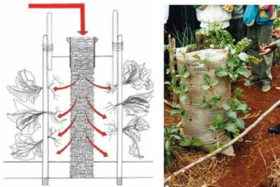
FIGURE 1. Sketch of a tower garden and photo of a bag garden.
