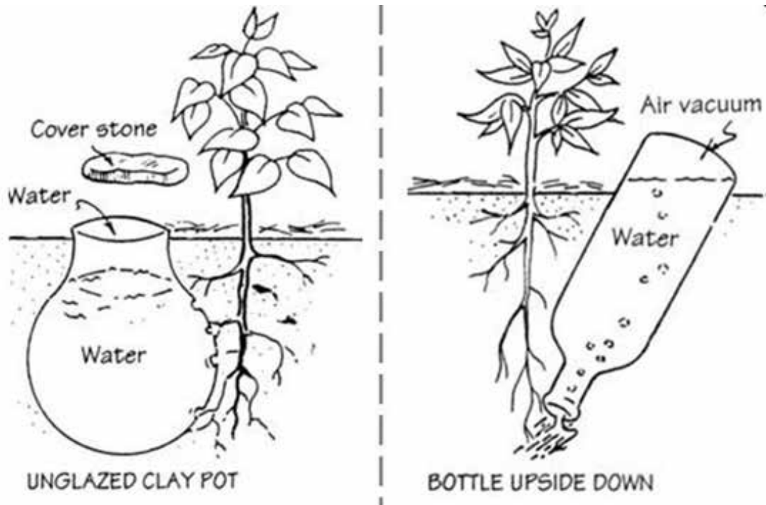
FIGURE 7. Sketch of clay pot and bottle irrigation.
