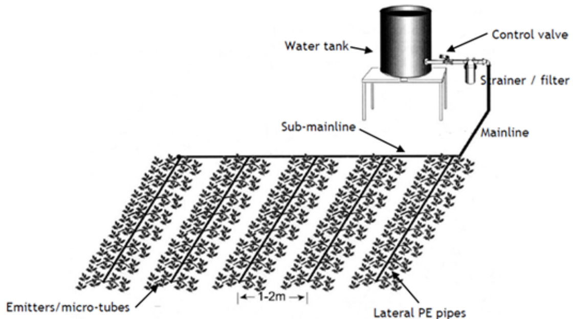
FIGURE 8. Sketch of bucket and drip irrigation kit.
