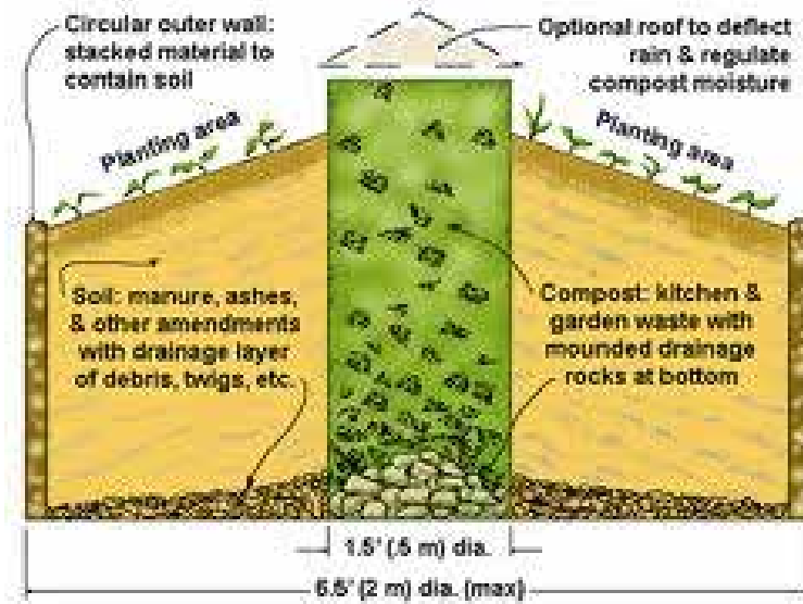
Keyhole Garden Cross-section A-A
