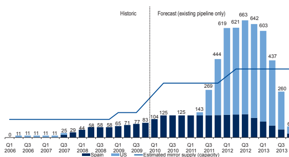
Figure 25. STEG project pipeline in US and Spain by quarter, MW
