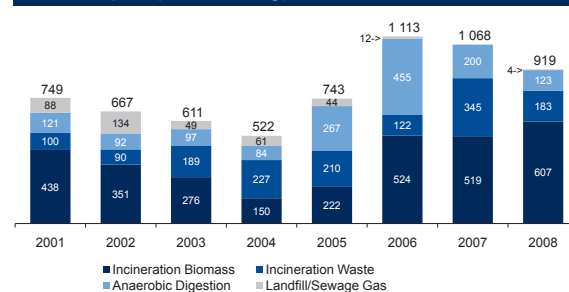
Figure 27. Commissioned Biomass & WtE capacity in Europe by technology 2001 to 2008, MW
