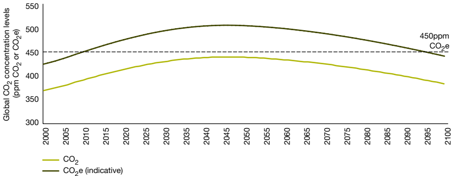
Figure 24: Global atmospheric concentration levels of CO 2
