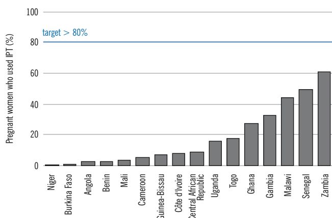
Fig. 4.15 Pregnant women who used IPT ( \geq 2 doses of SP/Fansidar; DHS, MICS, and MIS surveys)
